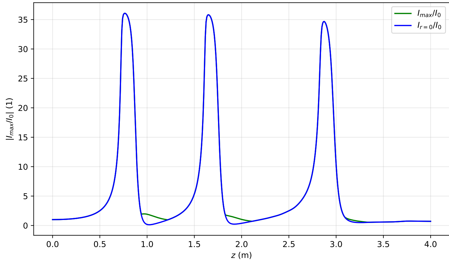
I_{\max}(x = 0, y = 0, z)/I_0 , \text{Pin}=3.0\text{Pcr} , artificial time
